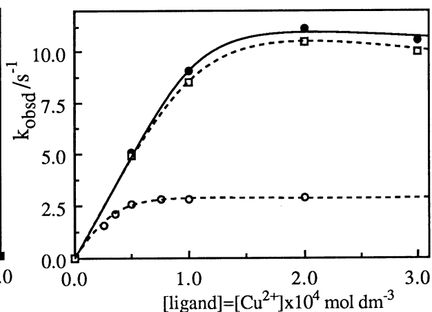
Fig. 4. Plots of rate constants vs. concentrations of ligand and Cu^{2+} ion for the transacylation of PNPP in SDS micelles; [ligand] = [Cu^{2+}] , [SDS] = 1 \times 10^{-2} \text{ mol dm}^{-3} ; \circ : 2 , \bullet : 3 at [PNPP] = 1.0 \times 10^{-5} \text{ mol dm}^{-3} , \square : 3 at [PNPP] = 2.0 \times 10^{-5} \text{ mol dm}^{-3} .
